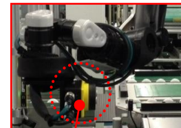
Inspection camera(Right)
