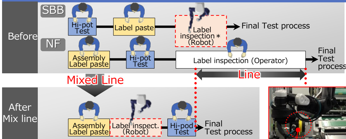
Inspection camera(Right)
